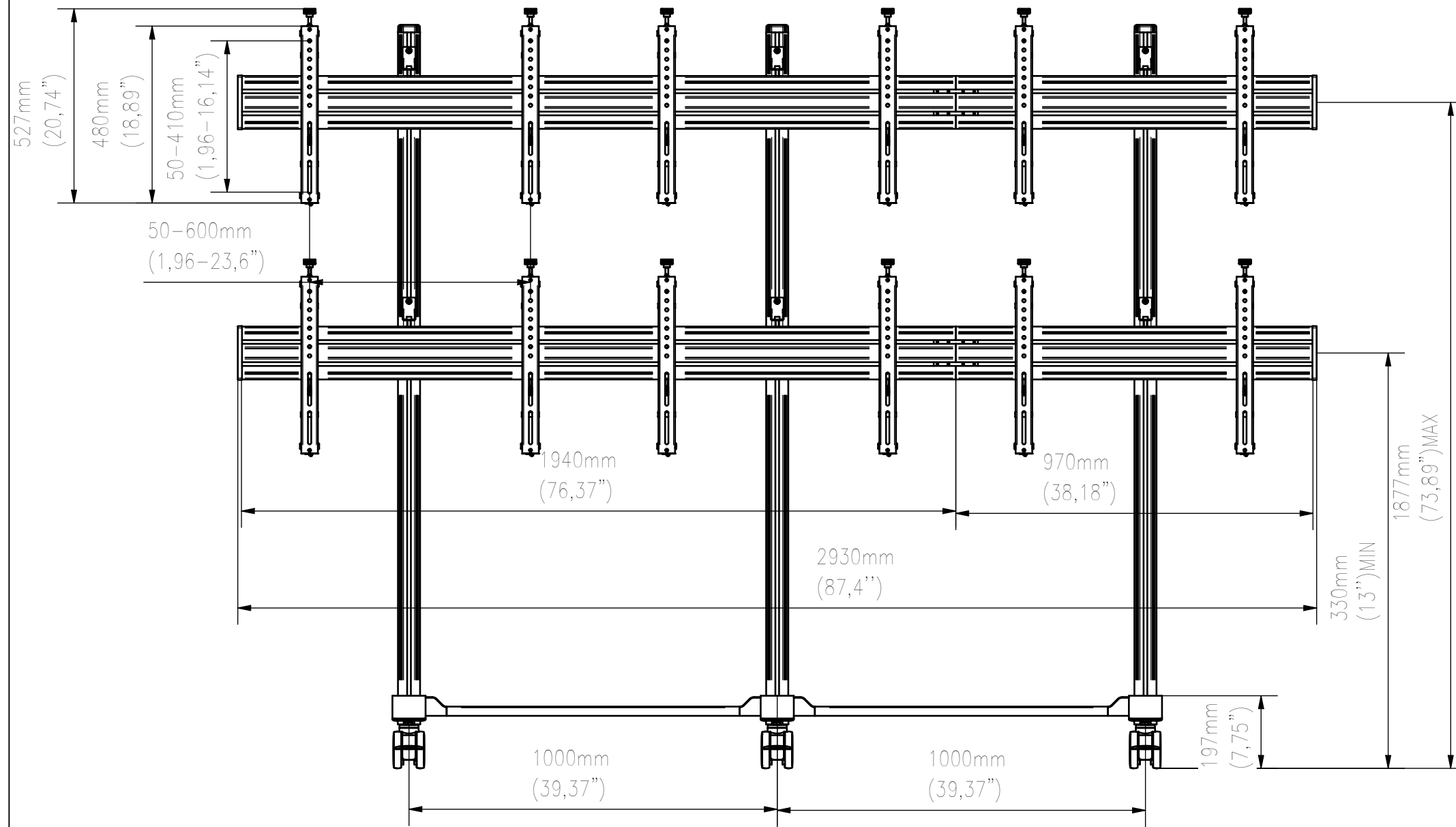
TOP VIEW
