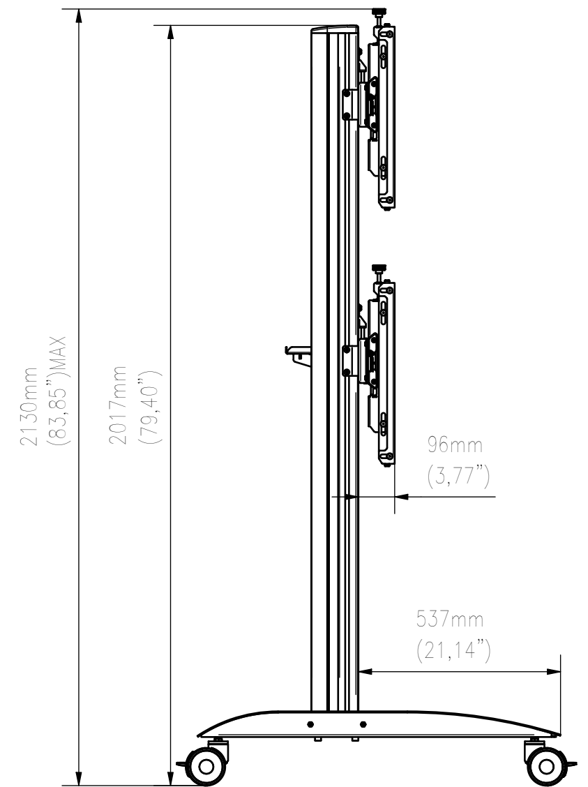
SIDE VIEW
