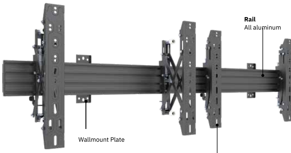
Exchangable Mounts Fixed, Tilt , Micro adjustment arms or Push in Pop out arms
