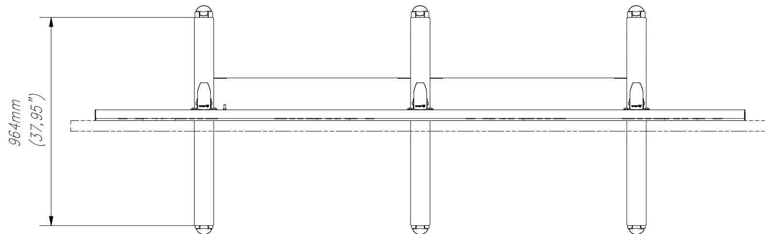
TOP VIEW
