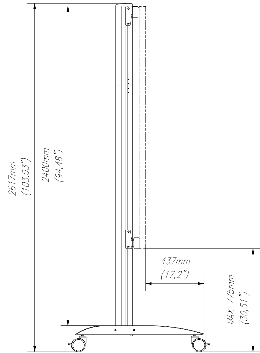
SIDE VIEW
