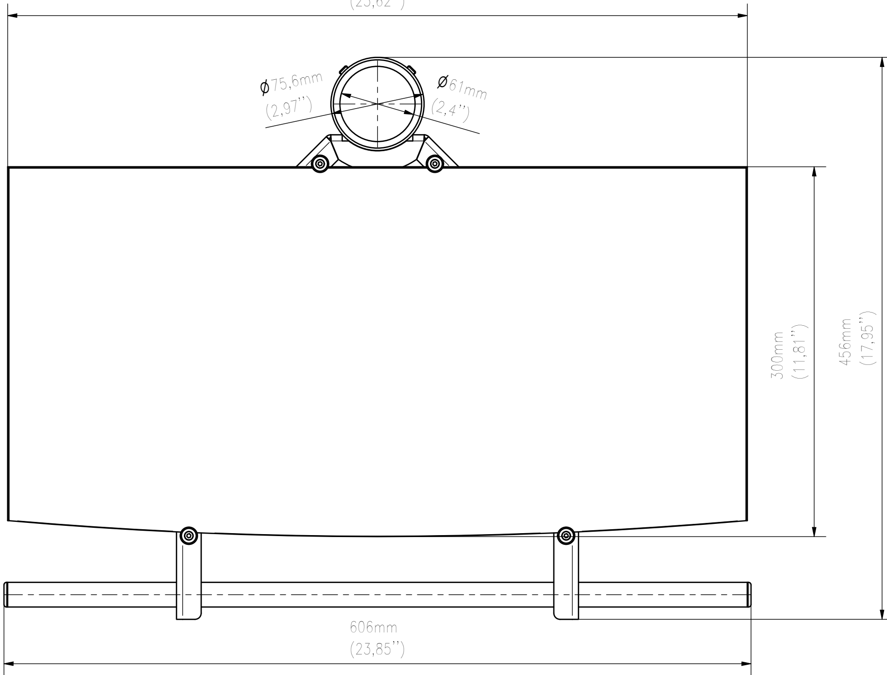
TOP VIEW
